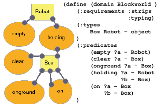
Figure 1: Declaration of language
