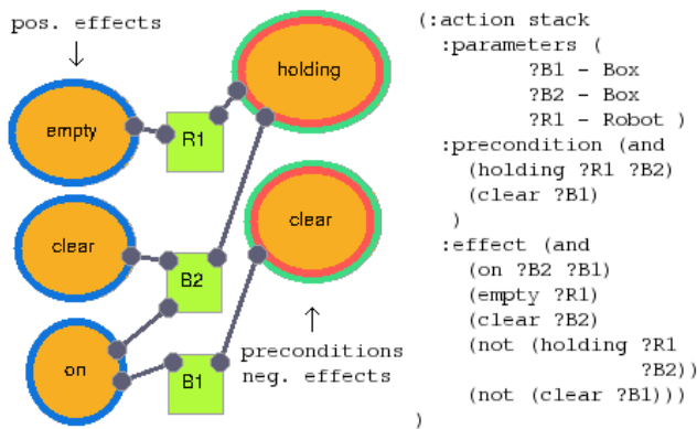
Figure 2: Planning operator example
