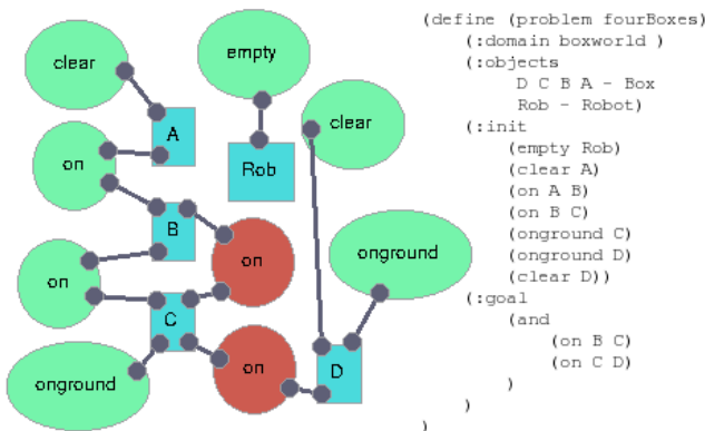
Figure 3: Planning problem example
